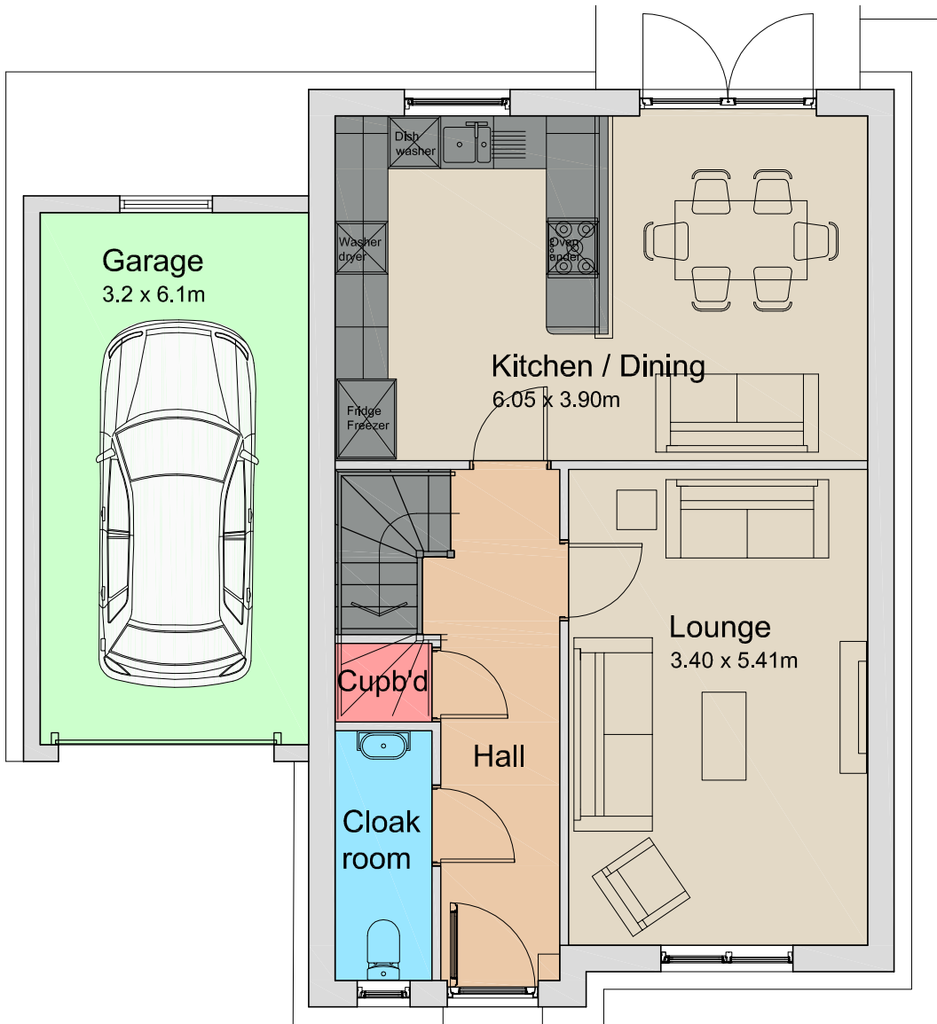
Ground Floor
