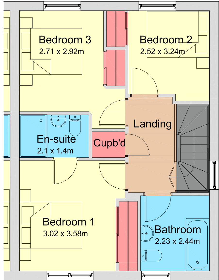
First Floor
